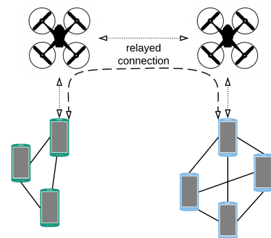
Fig. 1: Message relaying over UAVs enables inter-island communication among fully separated network islands.
